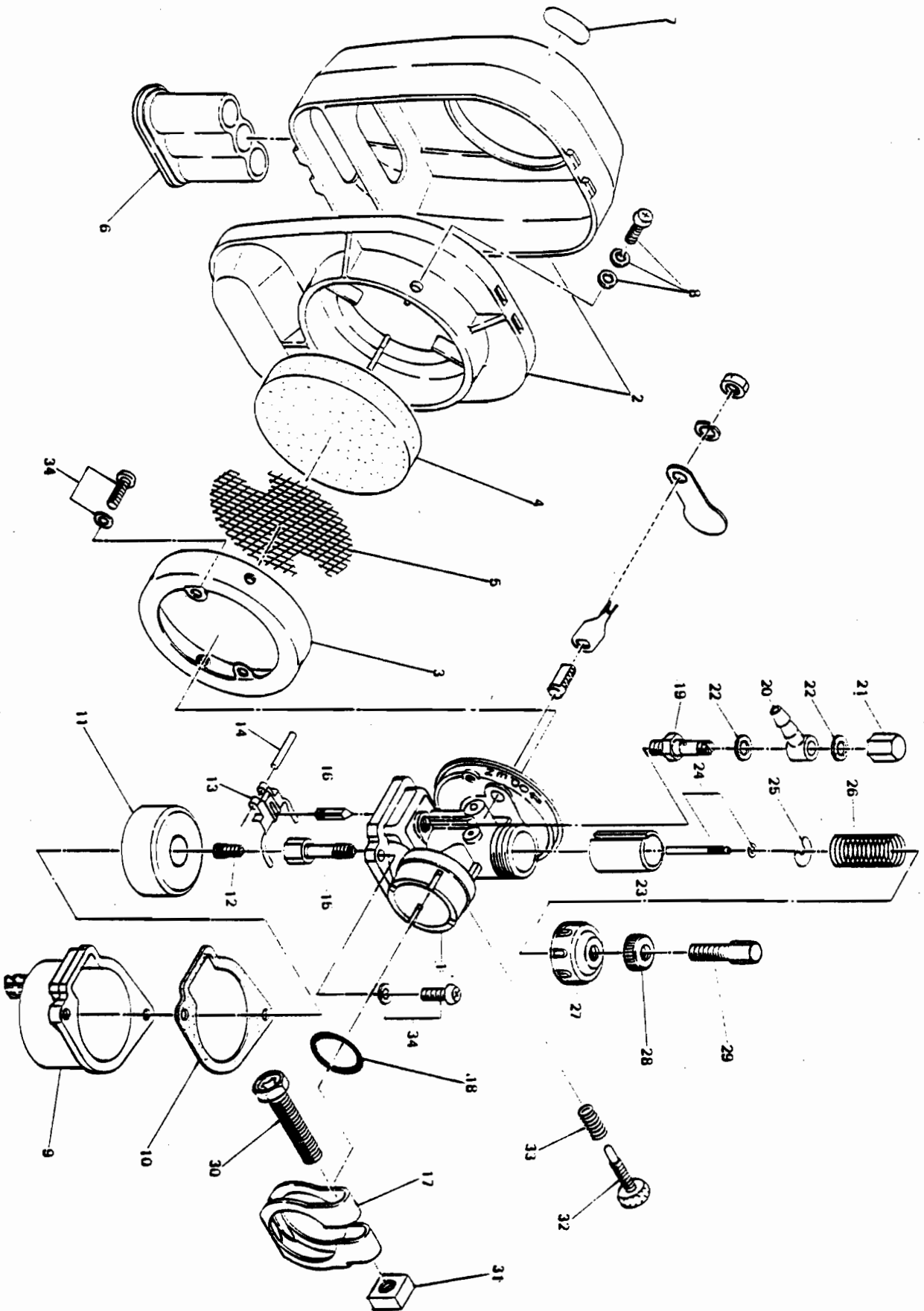
EC02A(RS02D-2) CARDURETOR
