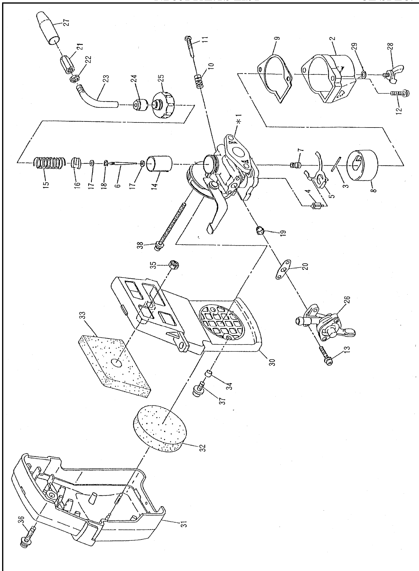
CARBURETOR & AIR CLEANER
