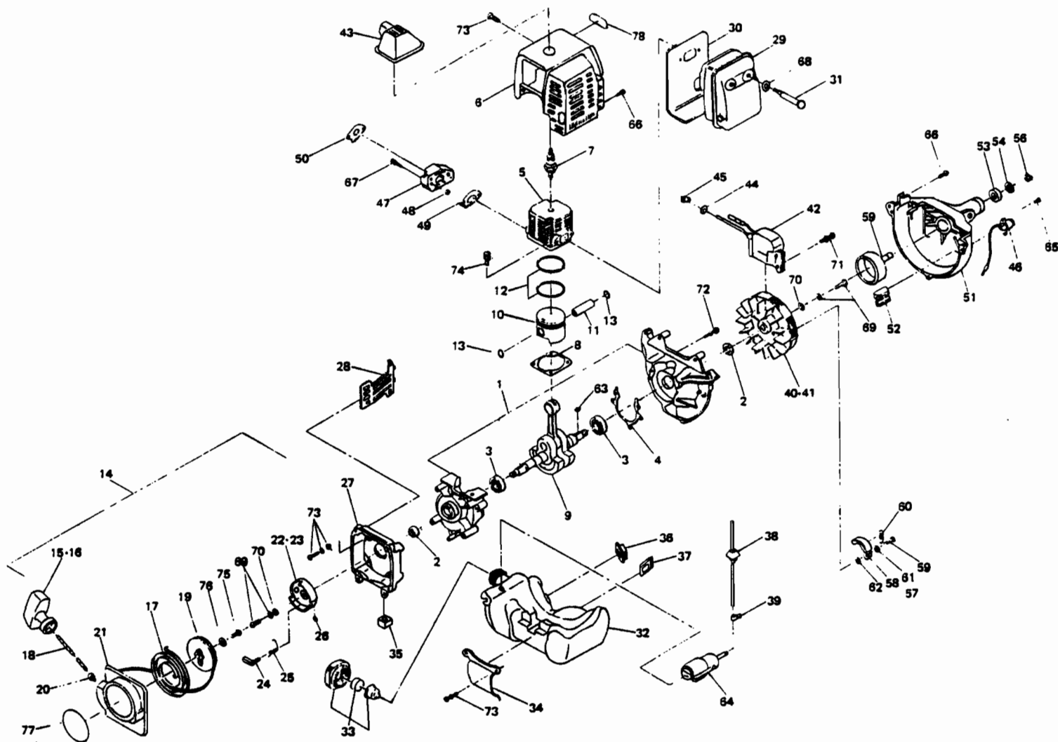
NB211 (A) ENGINE BODY
