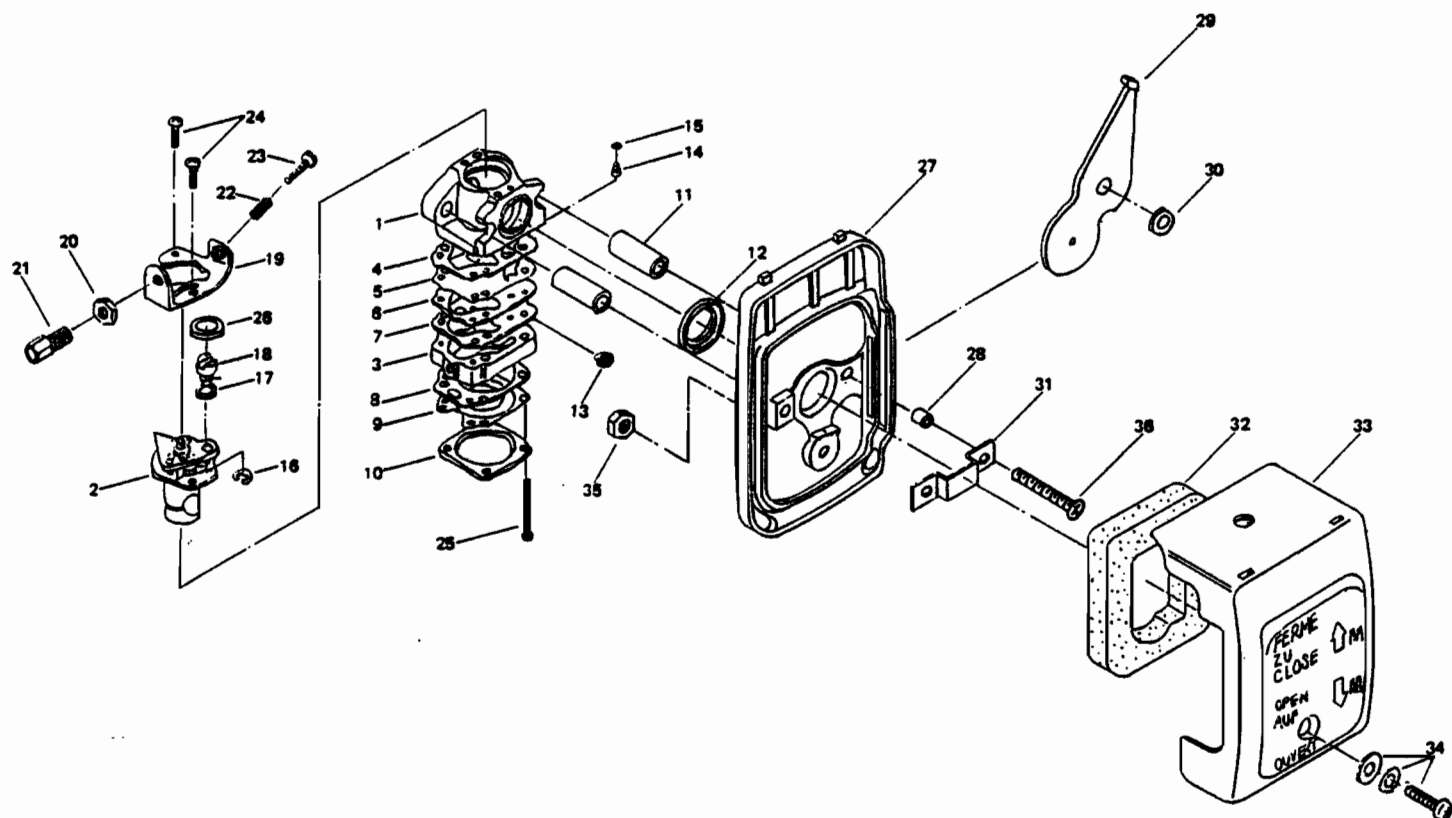
NB211 (A) CARBURETOR REPLACEMENT PARTS LIST
